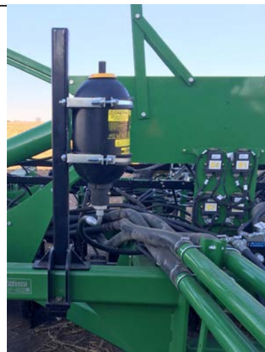
Accumulator on 60-ft w/ TBT cart. On 50-ft drills, accumulator must be far enough away from midline to avoid being struck by dolly wheels of wings when folded.
