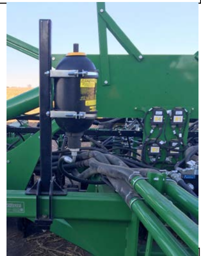
Accumulator on 60-ft w/ TBT cart. On 50-ft drills, accumulator must be far enough away from midline to avoid being struck by dolly wheels of wings when folded.
