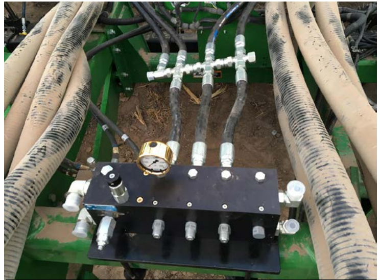
Photo M. Manifold installed on a 60-ft drill with TBT cart. 3 cartridges used, so 3 short feeder hoses going into 4 long 222" feeders, with places for 2 accumulators to plumb into the ends of equalizer fittings.
